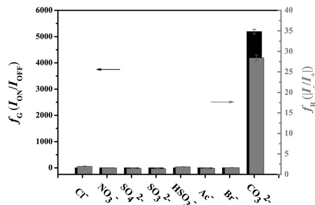
Figure 3. Selectivity of the carbonate-activated nanofluidic diode with the following parameters: d_{\text{tip}} = 24 nm, 1 M KCl, and 25 °C. f_G (black column and the left axis) and f_R (gray column and the right axis) of APTE-modified single nanochannel by treating with 1 M KCl, KNO 3 , K 2 SO 4 , K 2 SO 3 , KHSO 3 , KOAc, KBr, and K 2 CO 3 for 1 h, respectively. The f_G and f_R values of the functional nanodevice show much higher values after treatment with K 2 CO 3 than with other salts.
